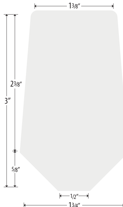
R Bar Plain End 14.2 lbs/ft | Lengths Available: 24", 27", 10'
