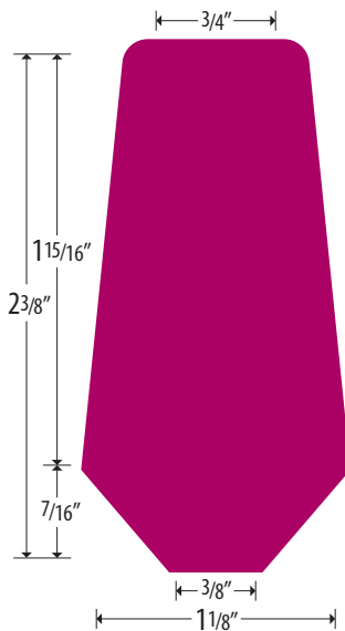
J Bar Pink End 7.4 lbs/ft
