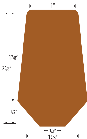
M Bar Copper End 8.7 lbs/ft
